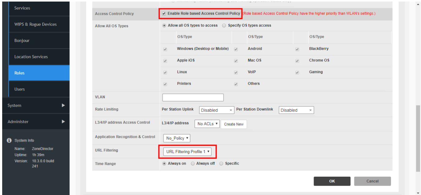
FIGURE 181 Applying a URL Filtering policy to a role
