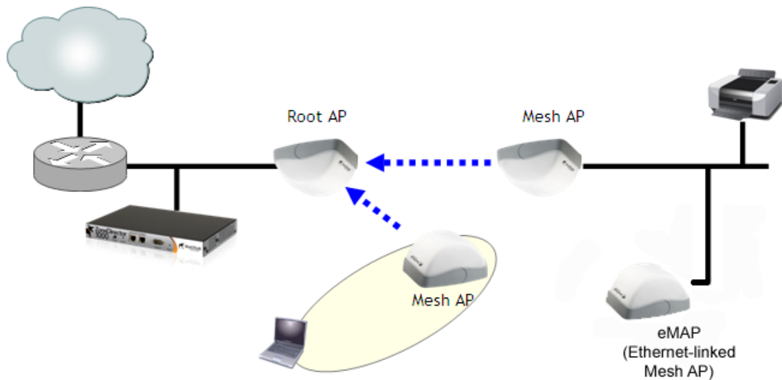
FIGURE 291 eMAP - Hybrid Mesh topology
