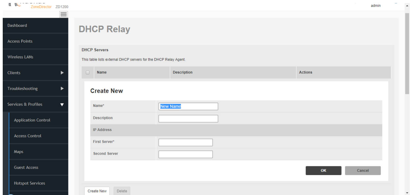
FIGURE 206 Creating a DHCP Relay server
