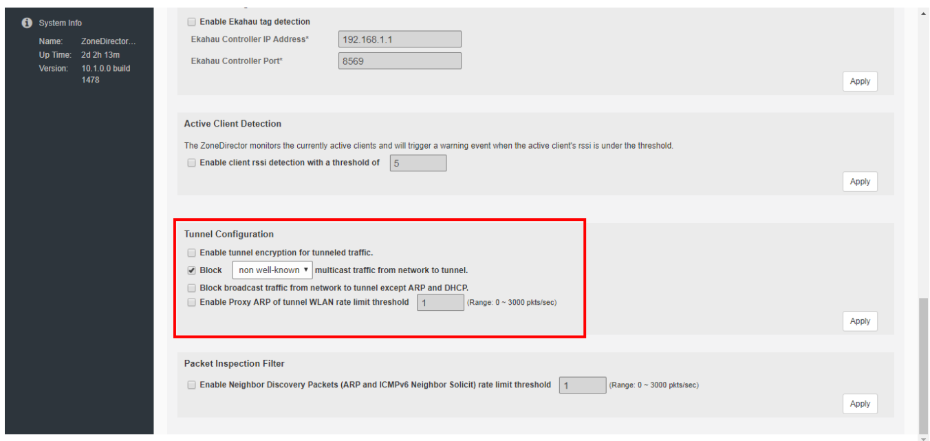
FIGURE 202 Set tunnel configuration parameters for all WLANs with tunnel mode enabled
