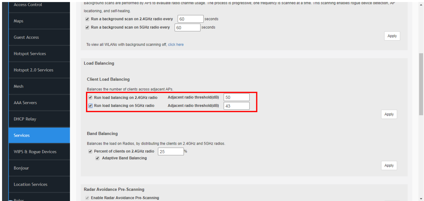
FIGURE 199 Enable Load Balancing globally
